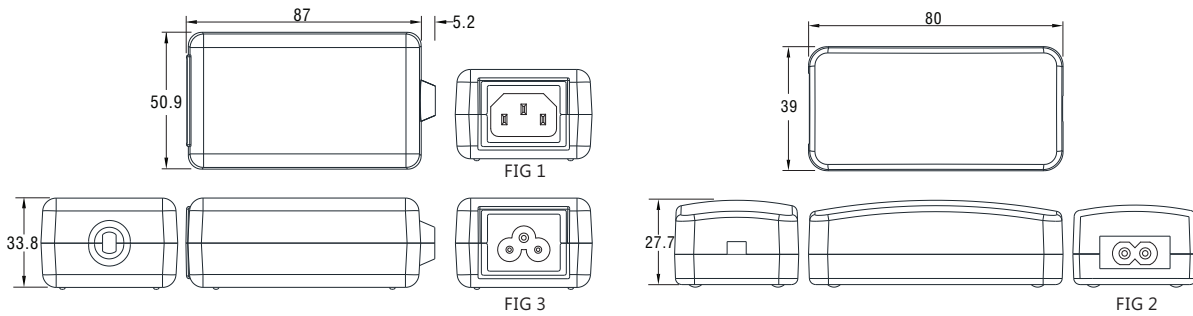
FIG 1: IEC-320-C14
