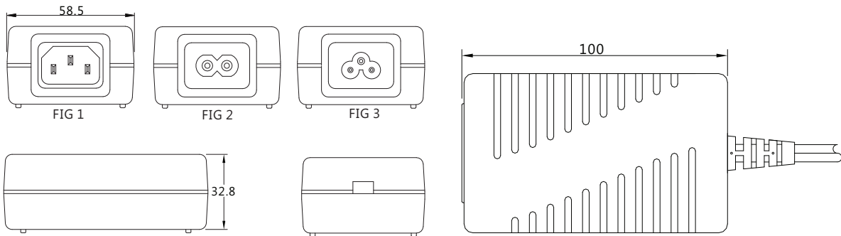
FIG 2: IEC-320-C8
