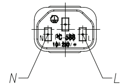
IEC-60320-C13
