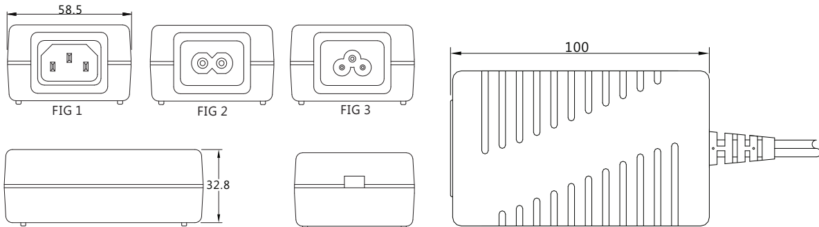
FIG 2: IEC-320-C8
