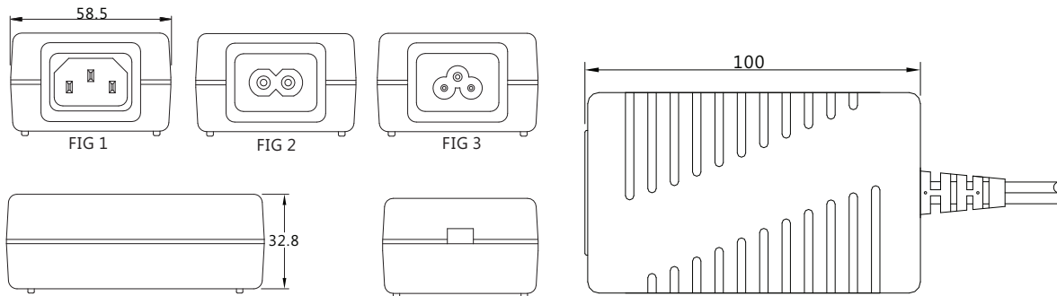
FIG 1: IEC-320-C14
