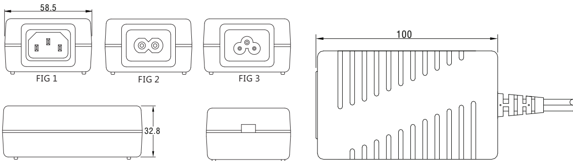
FIG 2: IEC-320-C8
