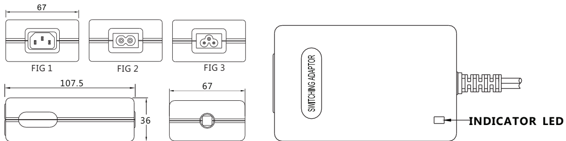
FIG 1: IEC-320-C14
